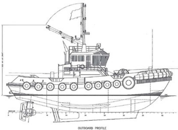
OUTBOARD PROFILE
