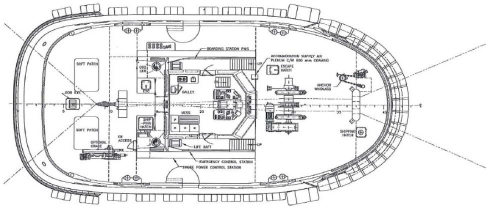
MAIN DECK PLAN
